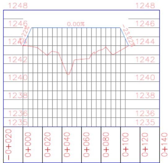
DAM AXIS PROFILE
